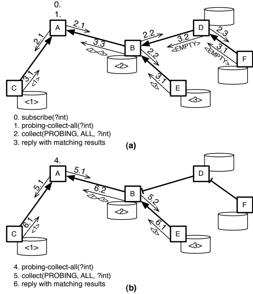
Figure 3: Arrows between nodes indicate routes for messages toward subscribers. (a) Without pruning, all probing-collect-all operations reach all hosts. (b) With pruning, subsequent probing-collect-all operations are limited to parts of the network with state. Nodes such as D whose descendants previously reported empty and have not since sent state changes (indicated by the T on the links) are eliminated from the request.
